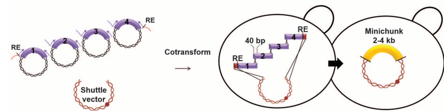
Fig. 2. SynIII construction. (A) BB synthesis. JHU students in the Build-A-Genome course synthesized 750-bp BBs (purple) from oligonucleotides. nt, nucleotides. (B) Assembly of minichunks. Two- to 4-kb minichunks (yellow) were assembled by homologous recombination in S. cerevisiae (table S1). Adjacent minichunks were designed to encode overlap of one BB to facilitate downstream assembly steps. Minichunks were flanked by a rare cutting restriction enzyme (RE) site, Xma I or Not I. (C) Direct replacement of native yeast chromosome III with pools of synthetic minichunks. Eleven iterative one-step assemblies and replacements of native genomic segments of yeast chromosome III were carried out by using pools of overlapping synthetic DNA minichunks (table S2), encoding alternating genetic markers ( LEU2 or URA3 ), which enabled complete replacement of native III with synIII in yeast.
