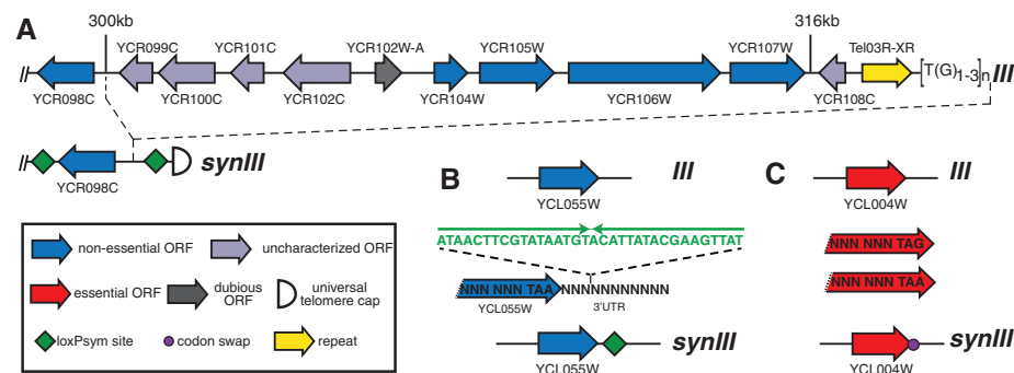
Fig. 1. SynIII design. Representative synIII design segments for loxPsym insertion ( A and B ) and stop codon TAG to TAA editing ( C ) are shown. Green diamonds represent loxPsym sites embedded in the 3' untranslated region (UTR) of nonessential genes and at several other landmarks. Fuchsia circles indicate synthetic stop codons (TAG recoded to TAA). Complete maps of designed synIII chromosome with common and systematic open reading frame (ORF) names, respectively, are shown in figs. S1 and S2.
