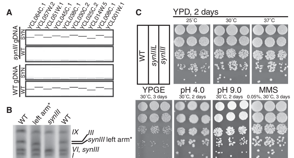
Fig. 3. Characterization and testing of synIII strain. (A) PCRTag analysis (one PCRTag per ~10 kb) of the left arm of synIII and WT yeast (BY4742) DNA is shown. Analysis of the complete set of PCRTags is shown in figs. S4 to S6. (B) Karyotypic analysis of synIII and synIIIIL strains by pulsed-field gel electrophoresis revealed the size reduction of synIII and synIIIIL compared with native III. Yeast chromosome numbers are indicated on the right side. SynIII (272,871 bp) and native chromosome VI (270,148 bp) comigrate in the gel. A karyotypic analysis of synIII and all intermediate strains is shown in fig. S8. (C) SynIII and synIIIIL phenotyping on various types of media. Tenfold serial dilutions of saturated cultures of WT (BY4742), synIIIIL, and synIII strains were plated on the indicated media and temperatures. YPD, yeast extract peptone dextrose; YPGE, yeast extract peptone glycerol ethanol; MMS, methyl methanesulfate. A complete set of synIII and synIIIIL phenotyping under various conditions is shown in fig. S11.
